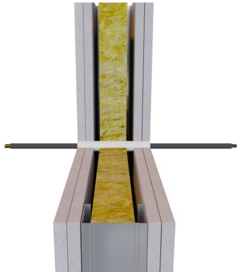
Figure A.1.1: Seal of a cable in a flexible wall.
