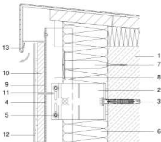
Figure A6.3: Roof edge (ventilated cladding system).
