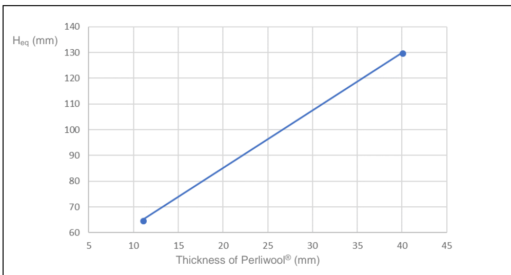
Figure A.2.2.6: Equivalent thickness of concrete (180 minutes).
