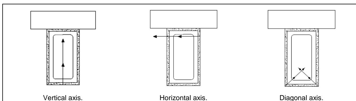
Figure A.2.2.1: Direction inside the concrete depth of a beam 12 .
