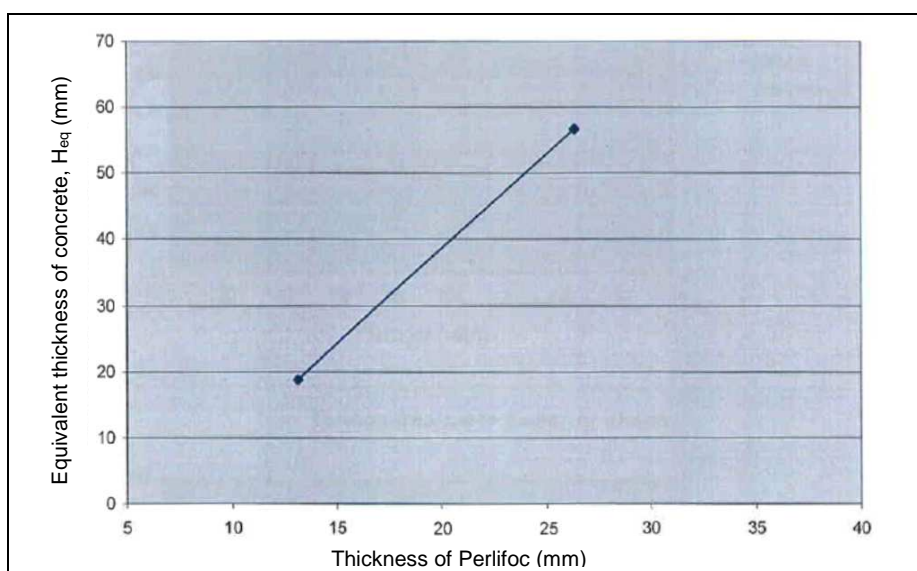
Figure A.3.4. Equivalent thickness ( H_{eq} ) vs thickness of Perlifoc® for a maximum temperature of 500 °C of the steel sheet.
